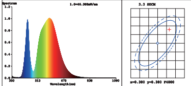
5700K(50W-Sensor)
