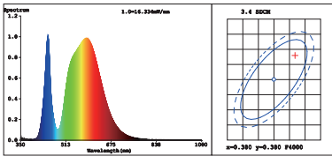
5700K(50W)
