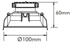
Cut-out: Ø88mm-90mm
