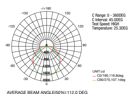
Luminous Intensity Distribution Diagram
