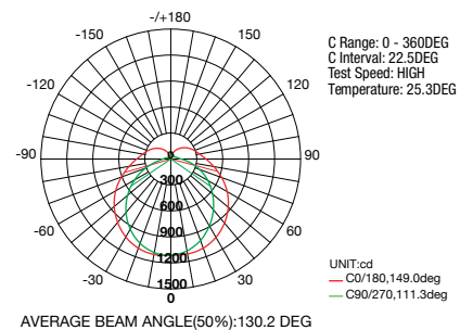
Product No: TLDB34640 Luminous Intensity Measure at 4000k CCT
