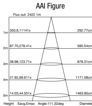
Product No: TLDB34640 AAI Figure at 4000k CCT
