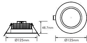
Cut-out: Ø90mm-120mm
